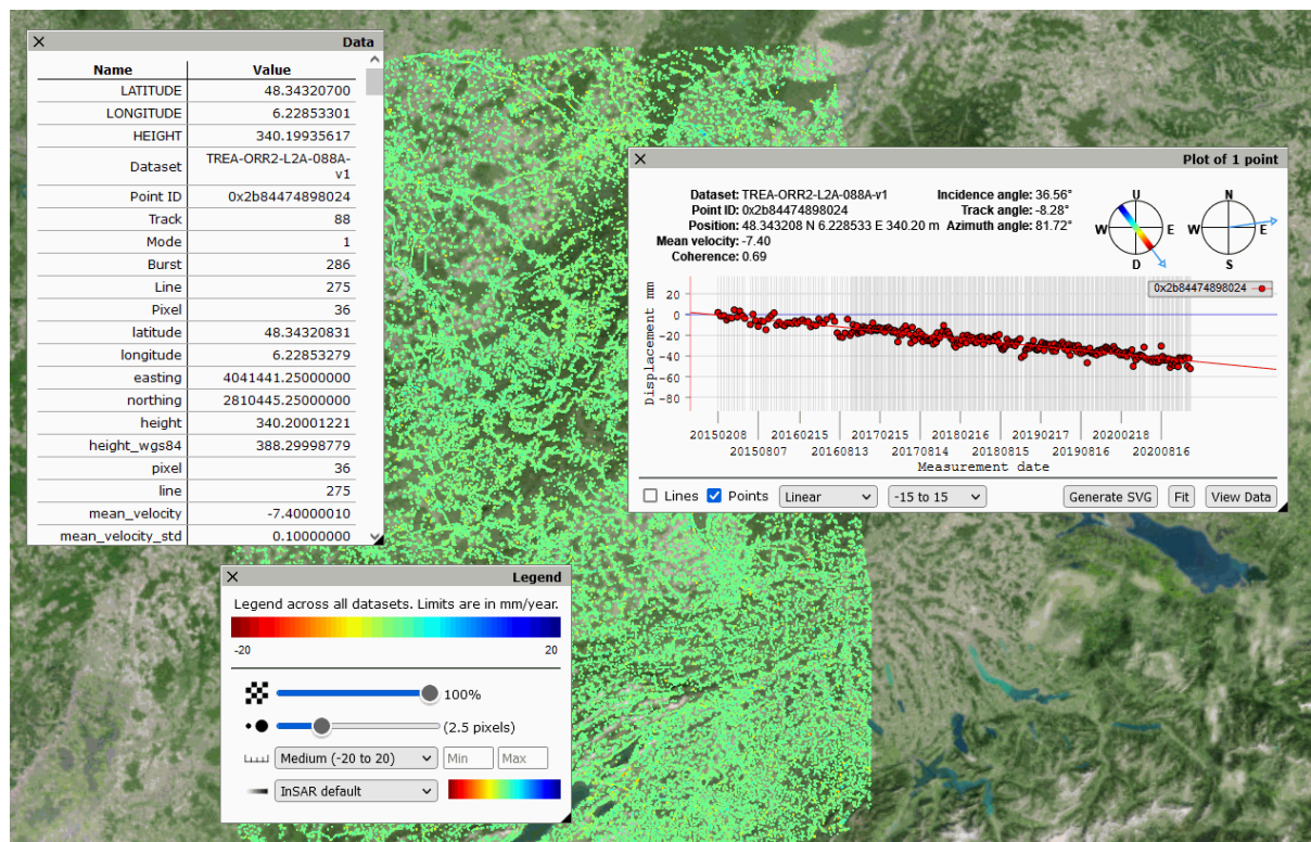
Figure 1: Figure 1 EGMS Basic (L2a) product. Provided as a 2D, colour-coded by average velocity, map. Displacement data provided in the satellite line-of-sight, and in radar geometry, with annotated geolocalisation and quality measures per measurement point. A time series plot is associated with each point.
