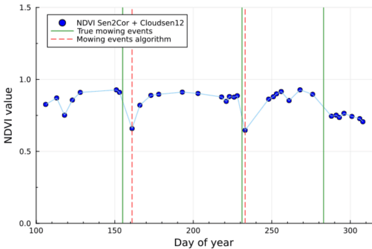
Figure 13: Figure 13: Single-pixel NDVI time series and mowing events (ground truth and detected) for 2021 (32TPT; WGS84 coordinates: 11.3103°E, 47.5884°N).
