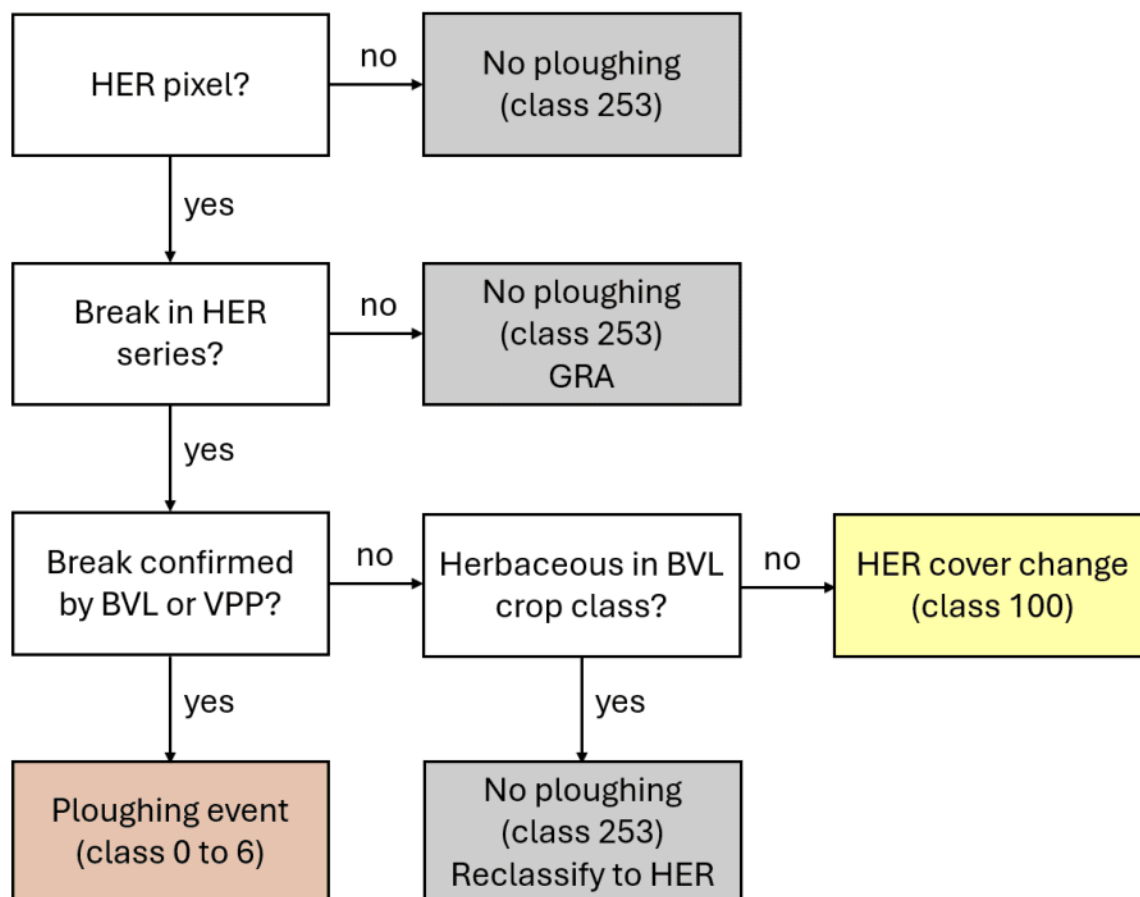
Figure 8: Figure 8: Flowchart of the PLOUGH decision logic
