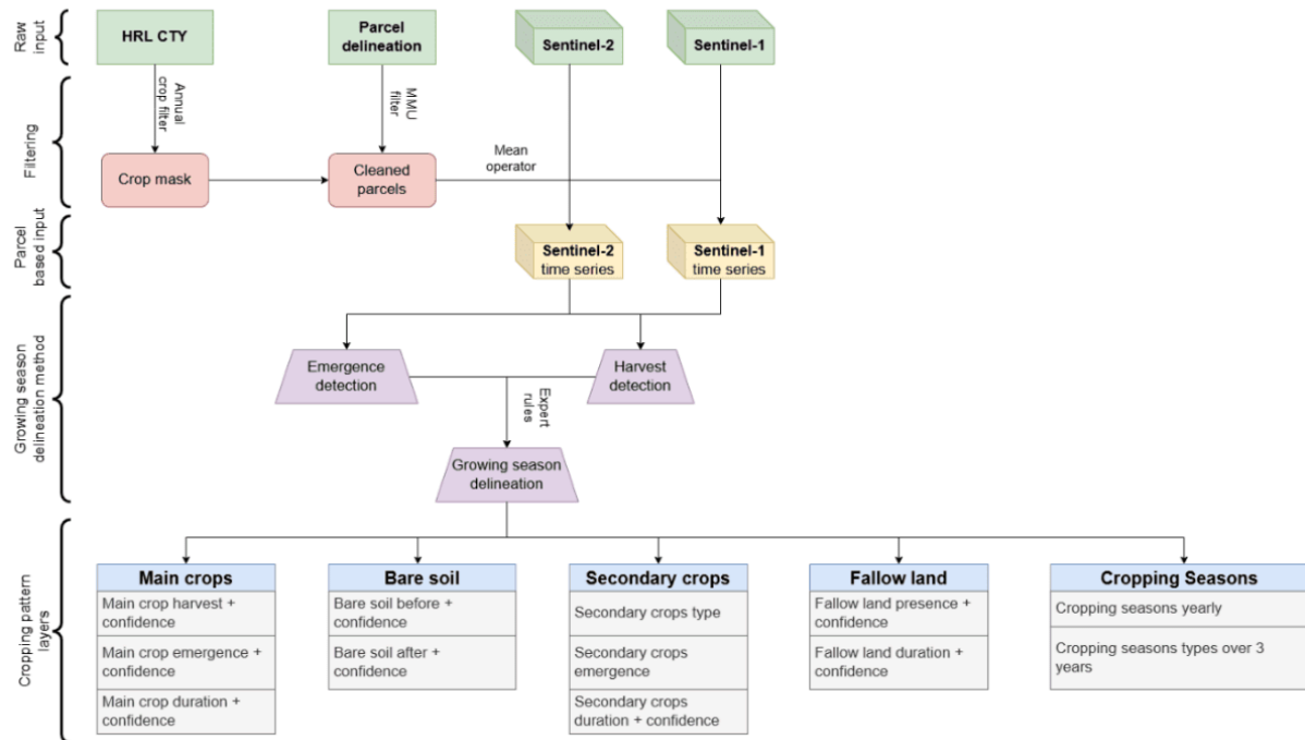
Figure 21: Figure 21: Schematic overview of cropping pattern products generation.
