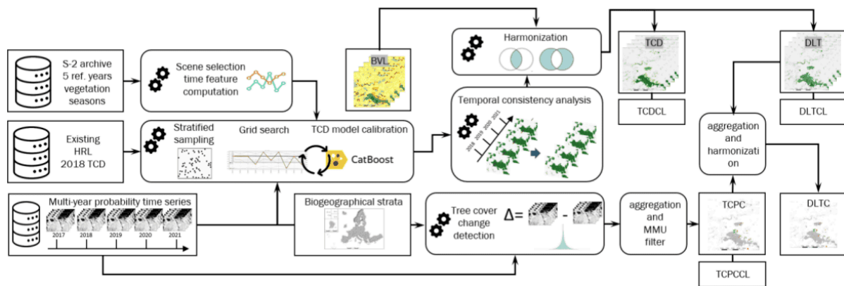
Figure 3: Figure 3: High-level flow chart of the production workflow for the Tree Cover & Forests products TCD, DLT, TCPC and DLTC.
