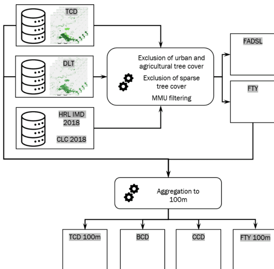
Figure 4: Figure 4: High-level flow chart of the production workflow for the Tree Cover & Forests products FADSL, FTY and aggregated products at 100m.
