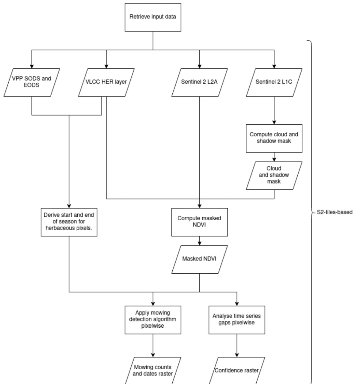
Figure 14: Figure 14: Processing workflow and pipeline for the GRAMD and GRAME layers part 1: Source data selection, pre-processing and cloud masking, and mowing event detection.
