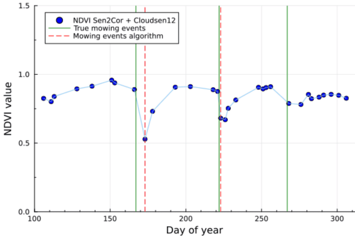
Figure 12: Figure 12: Single-pixel NDVI time series and mowing events (ground truth and detected) for 2021 (32TPT; WGS84 coordinates: 11.3151°E, 47.5911°N).
