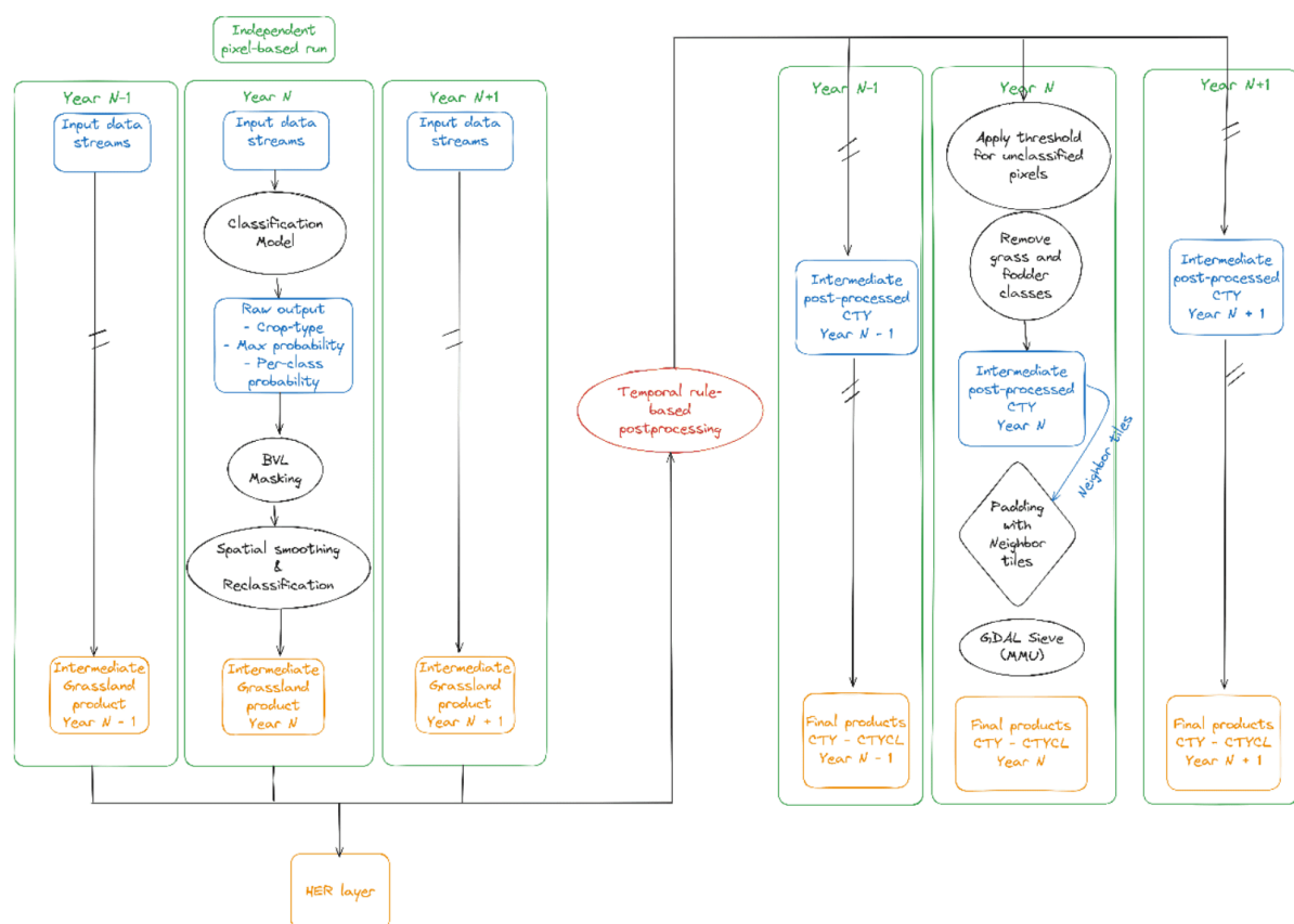
Figure 19: Figure 19: CTY postprocessing pipeline flowchart
