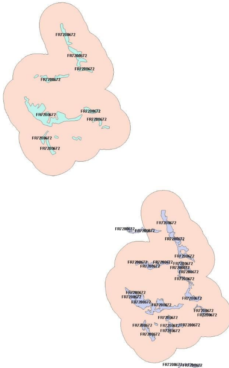
Figure 8 - Example of Natura 2000 DB site changes from 2015 (top) to 2018 (bottom). Background N2K AOI
