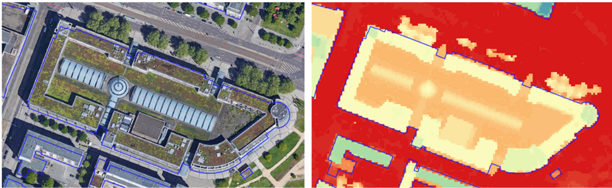
Figure 6-18 Satellite imagery (left) and DSM at half meter resolution (right)
