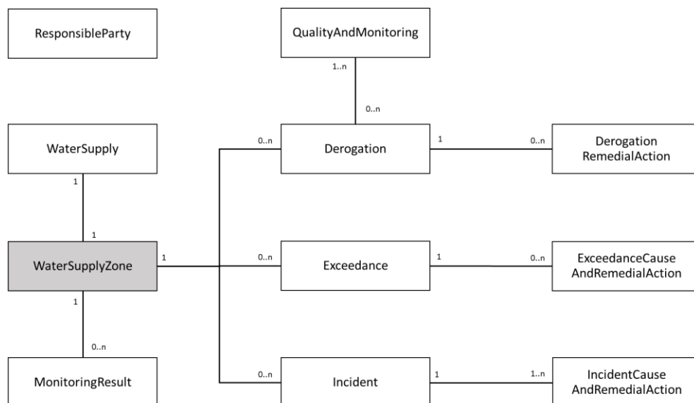
Figure 1: Reporting tables and main relationships between tables.
