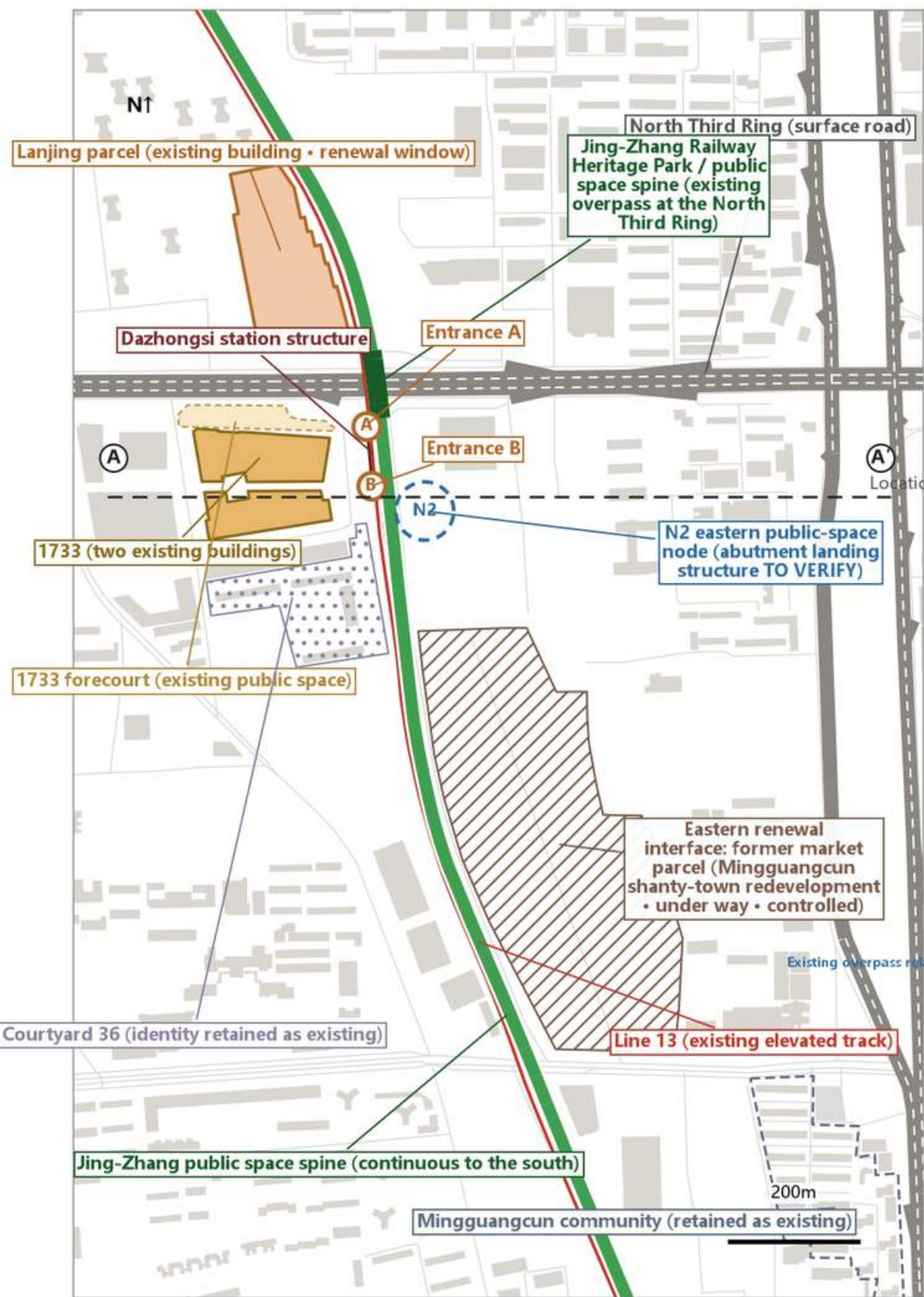
T1 site fact plan | existing objects (OSM) + verified positions of the station structure, entrances A/B and 1733
