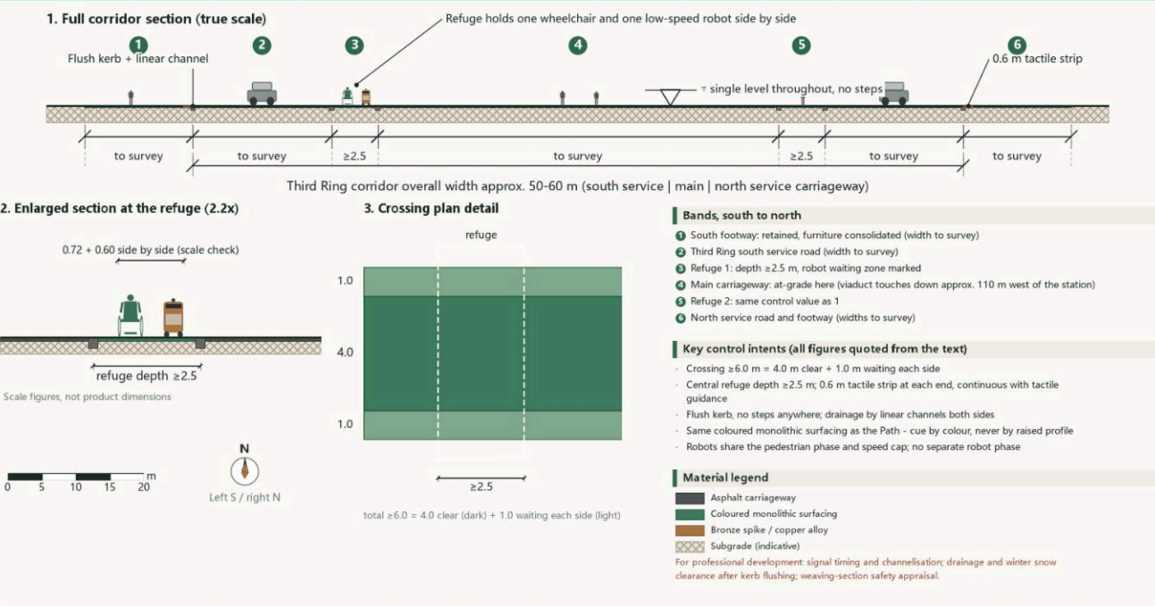
Section DZS-1 · Soundwave Path crossing an urban road (conceptual section)
