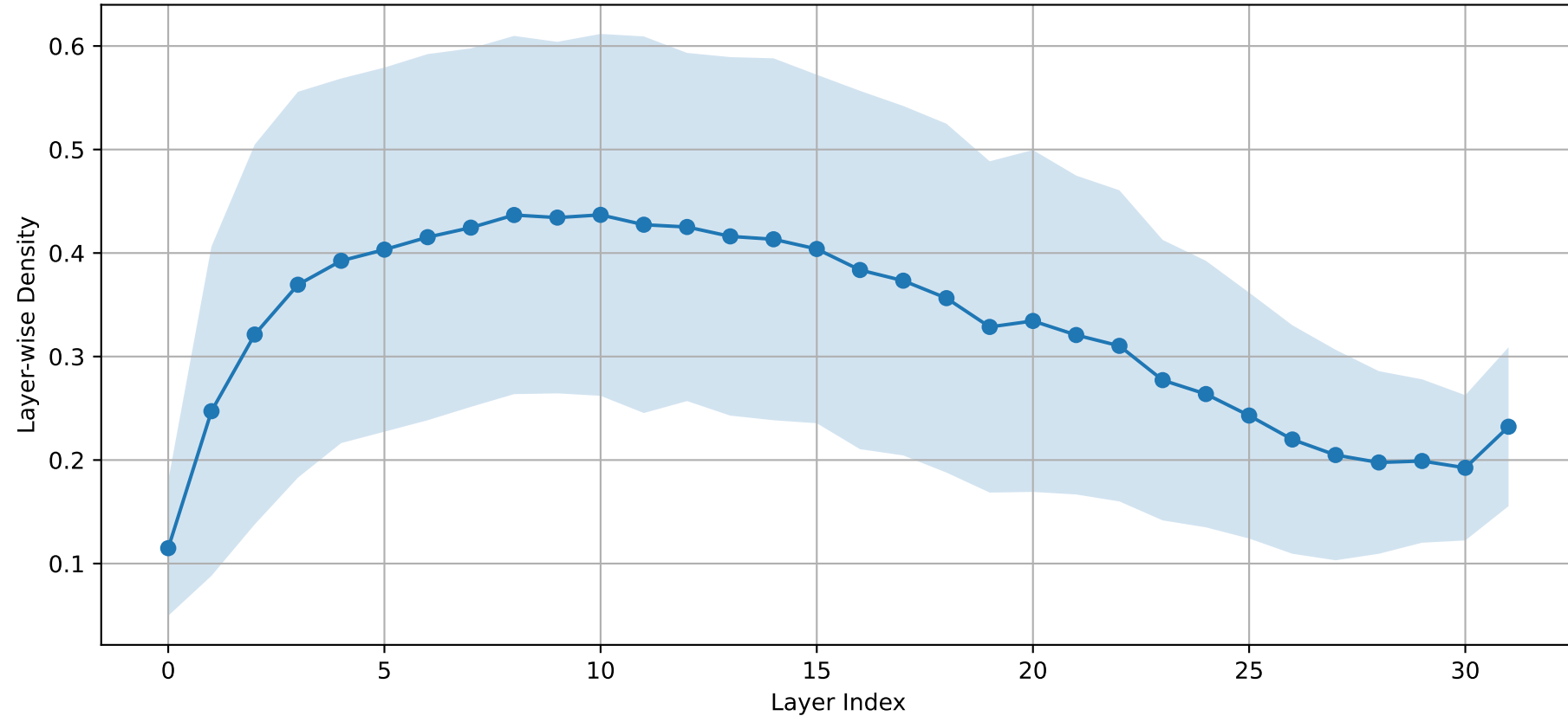
Meta-Llama-3.1-8B-Instruct Overall Layer-wise Score \rho^{(\ell)}
