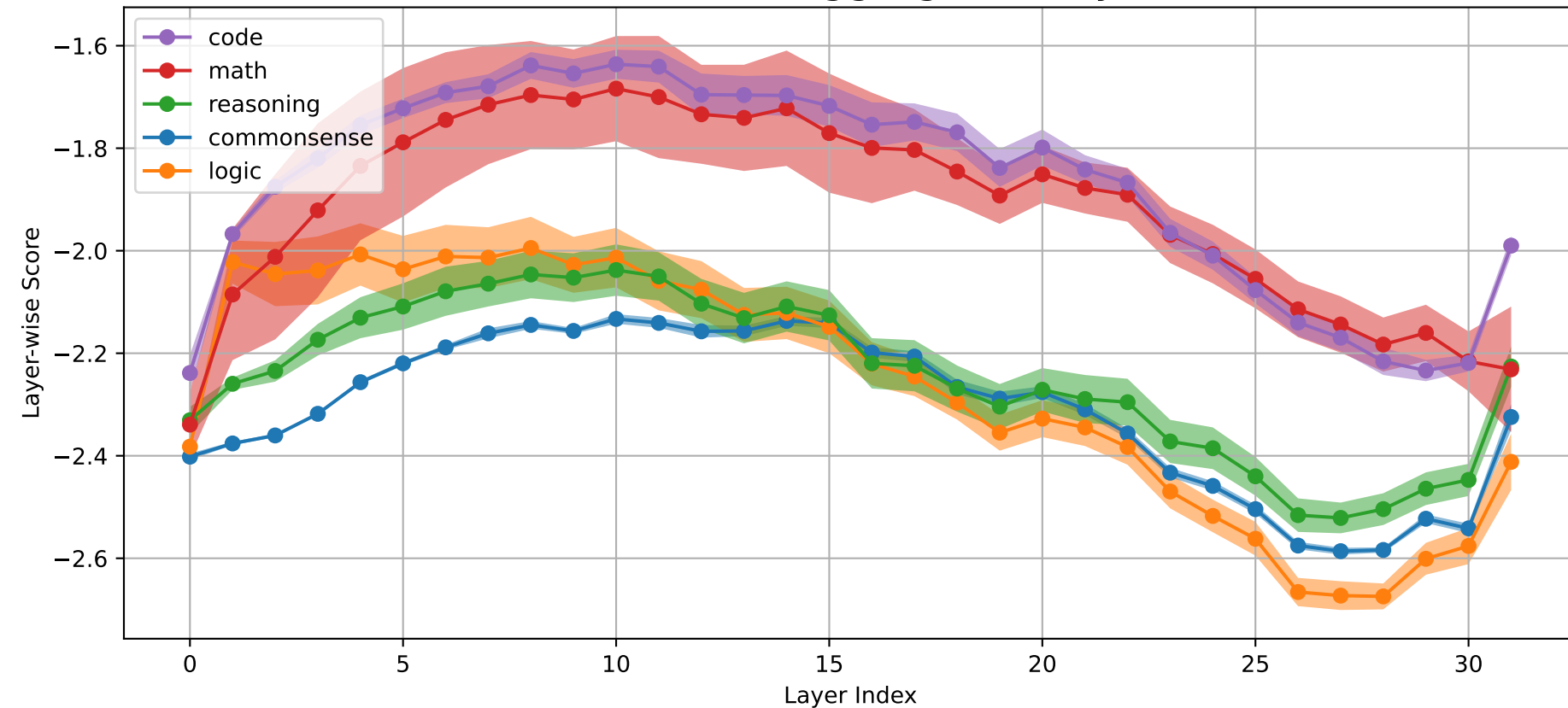
Llama-3.1-8B-Instruct Task Aggregated Layer-wise Score S^{(\ell)}
