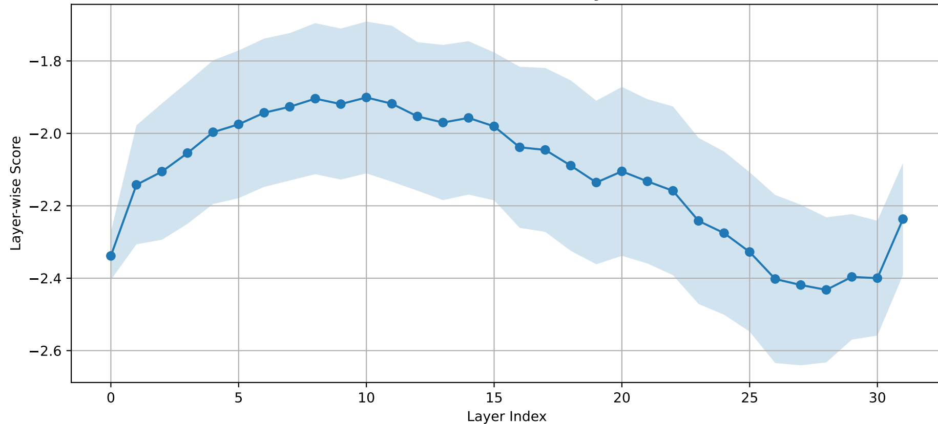
Llama-3.1-8B-Instruct Overall Layer-wise Score S^{(\ell)}
