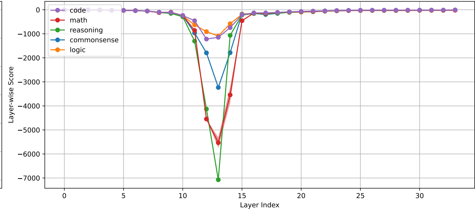
Gemma-3-4b-it Task Aggregated Layer-wise Score S^{(\ell)}
