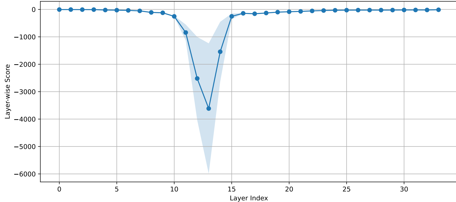
Gemma-3-4b-it Overall Layer-wise Score S^{(\ell)}
