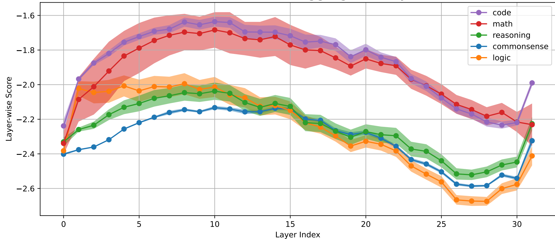
Meta-Llama-3.1-8B-Instruct Task Aggregated Layer-wise Score S^{(\ell)}
