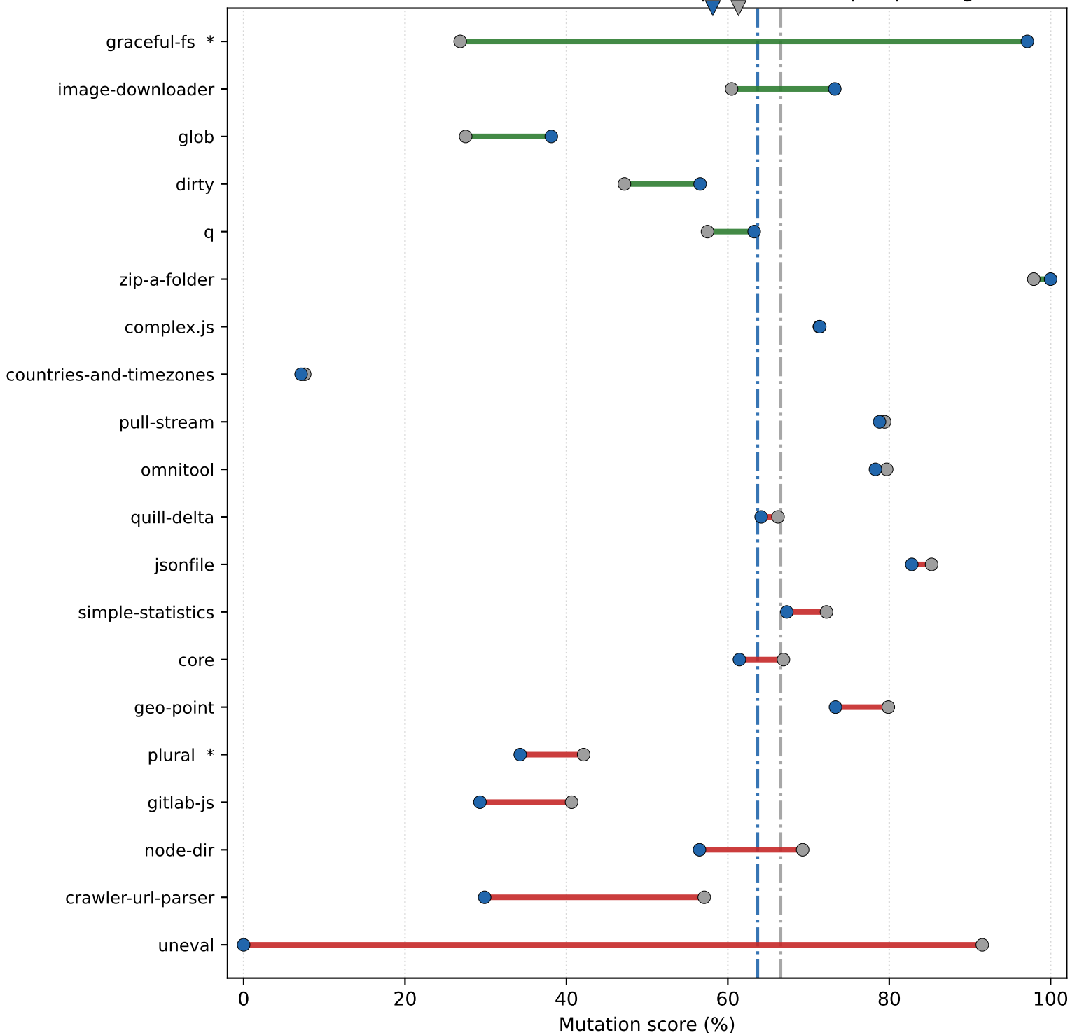
Hidden vs. full mutation feedback (pre-residual) per package
