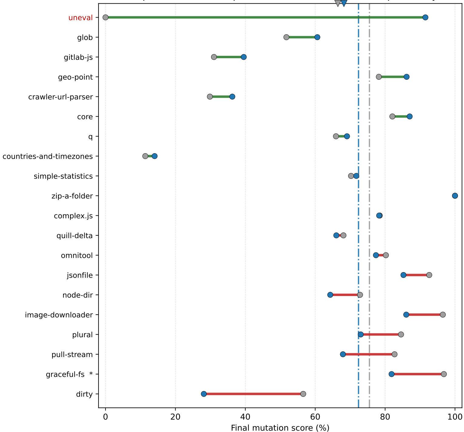
Temperature 0 vs. temperature 1 final mutation score per library
