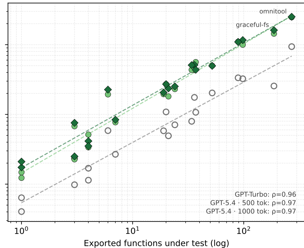
vs. functions under test
