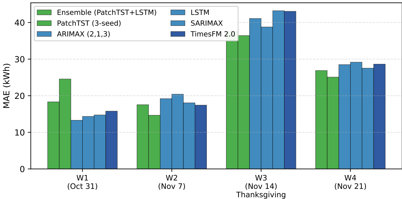
Per-window MAE -- window 3 (Thanksgiving) is hard for every model
