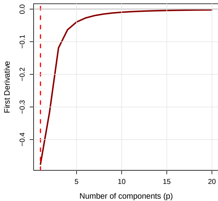
Bad Boundaries: \Delta_1
