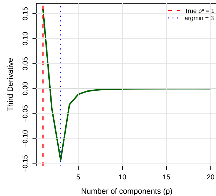
Bad Boundaries: \Delta_3
