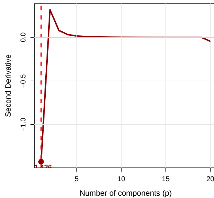
Bad Boundaries (assumes M_p[0]=0 ): \Delta_2
