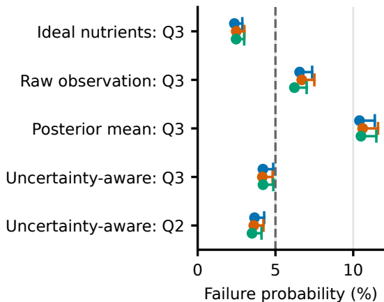
(c) Noise 0.5 SD, A
