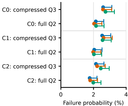
(c) Noise 0.5 SD, A
