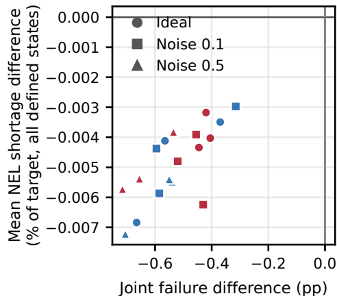
b Full pool: measurement
