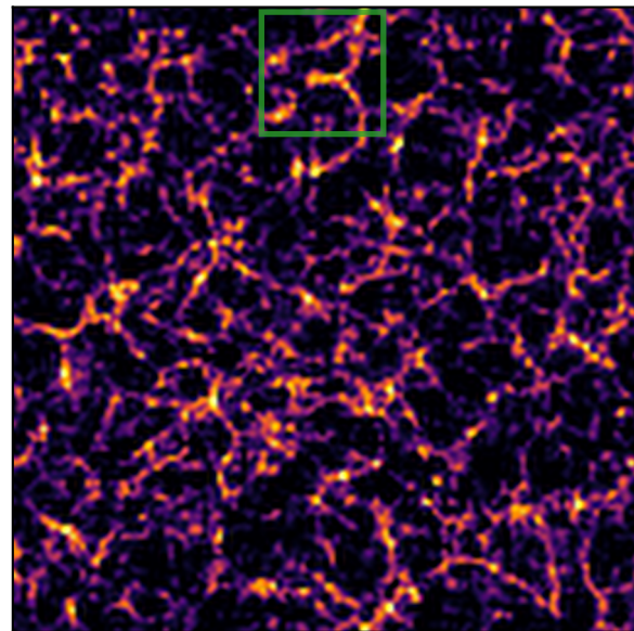
PM-SO
