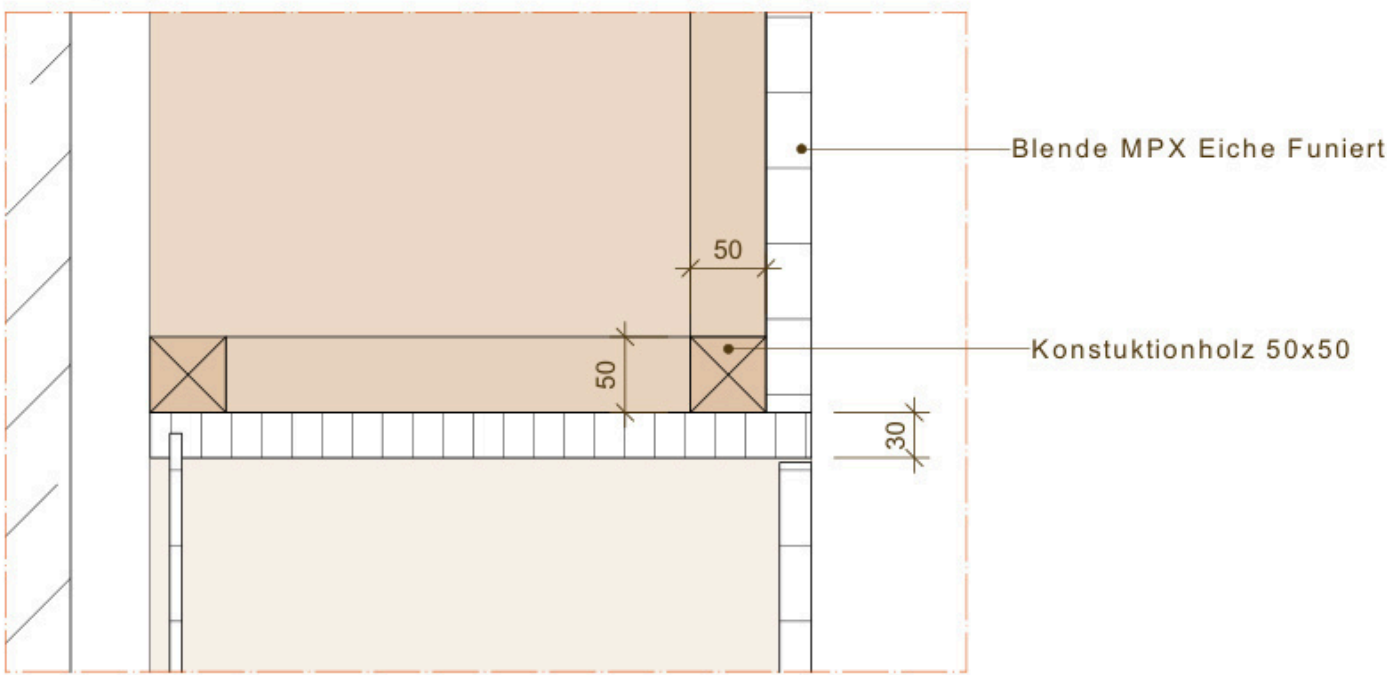
Blende Detail 8 M 1:5
