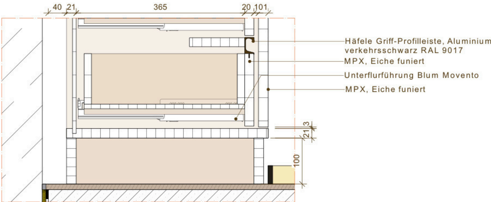
Sockel Detail 7 M 1:5
