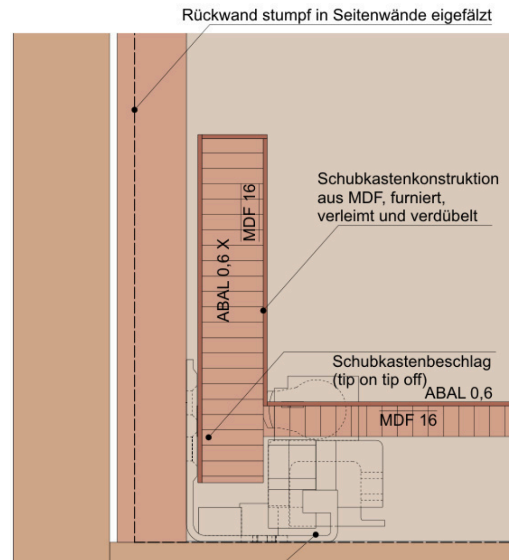
Detail TIP ON TIP OFF M1:1
