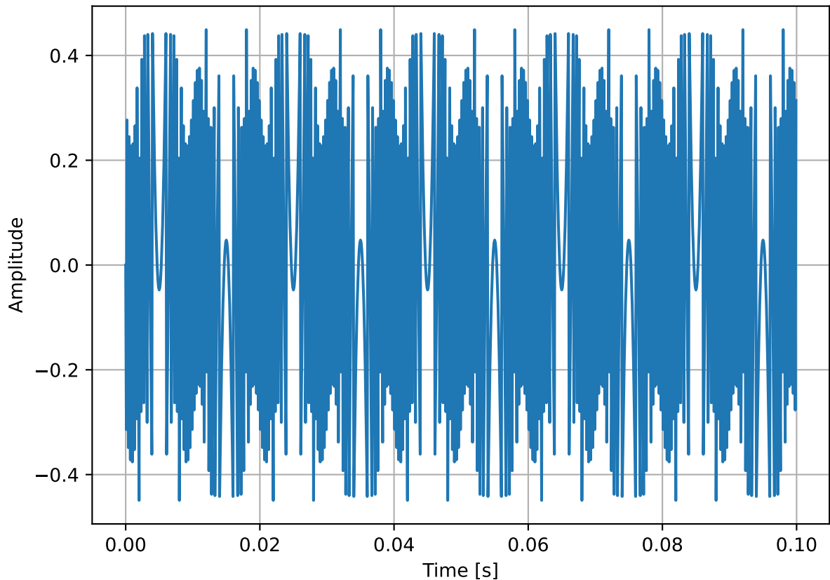
Quantized Sine Wave Error
