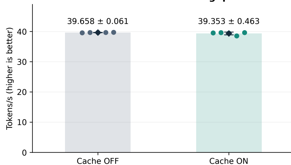
Generated-token throughput
