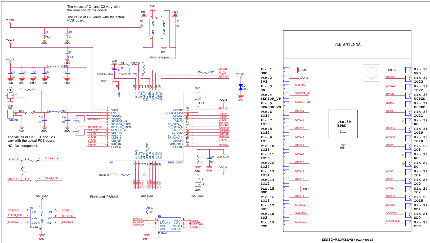
Figure 5: ESP32-WROVER-B Schematics
