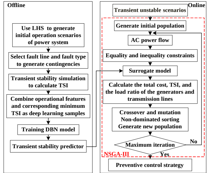
Fig. 3. Proposed DBN based surrogate model for preventive control.
