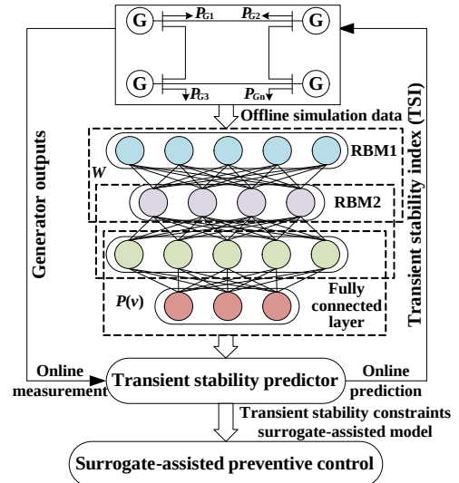
Fig. 1. DBN based surrogate model for multi-objective TSC-OPF.
