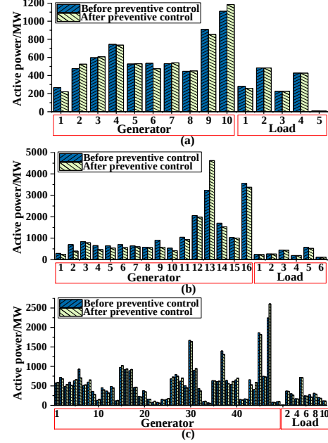
Fig. 11. Generator redispatch results considering load shedding. (a) 39-bus system. (b) 68-bus system. (c) 140-bus system.
