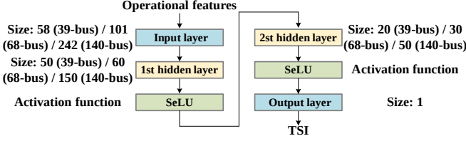
Fig. 5. The structure of proposed DBN-based transient stability predictor.
