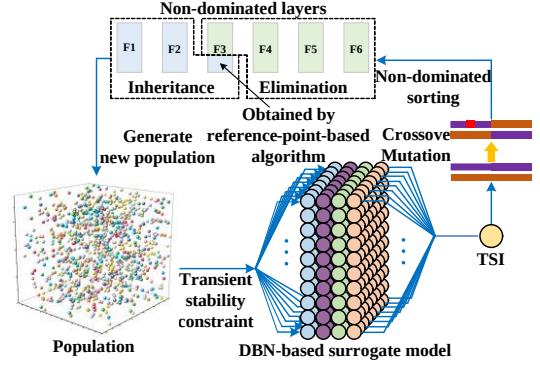
Fig. 2. Proposed surrogate model assisted preventive control using NSGA-III algorithm.
