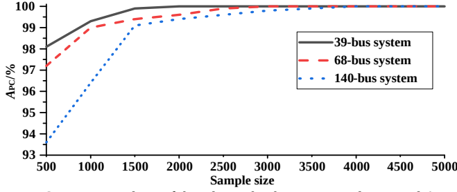
Fig. 4. Sensitivity analysis of the relationship between sample size and A_{PC} .
