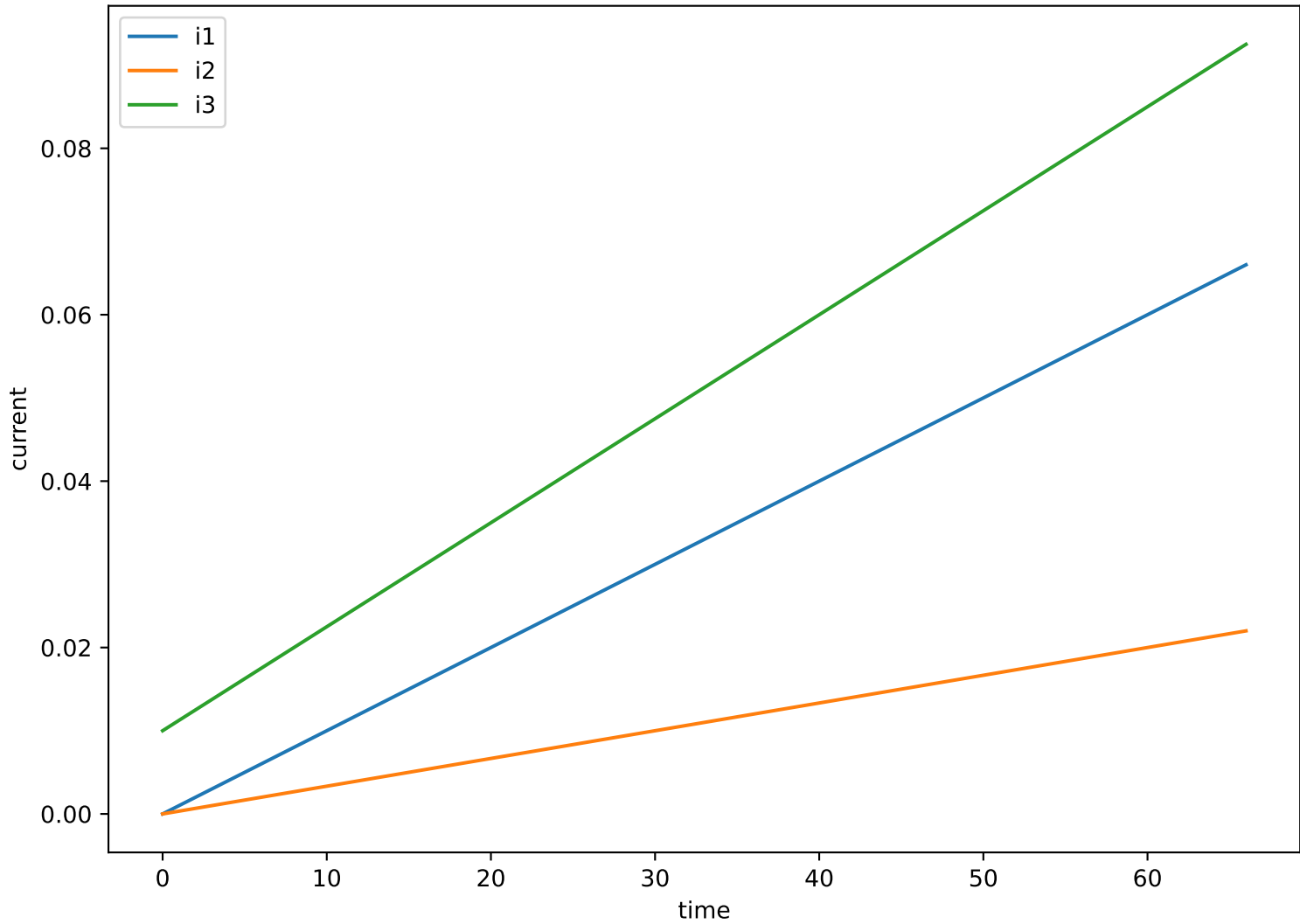
Currents (lemniscate)
