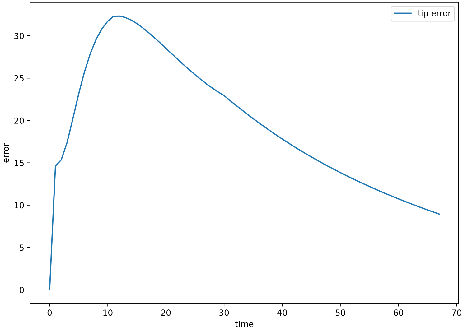
Tip tracking error (lemniscate)
