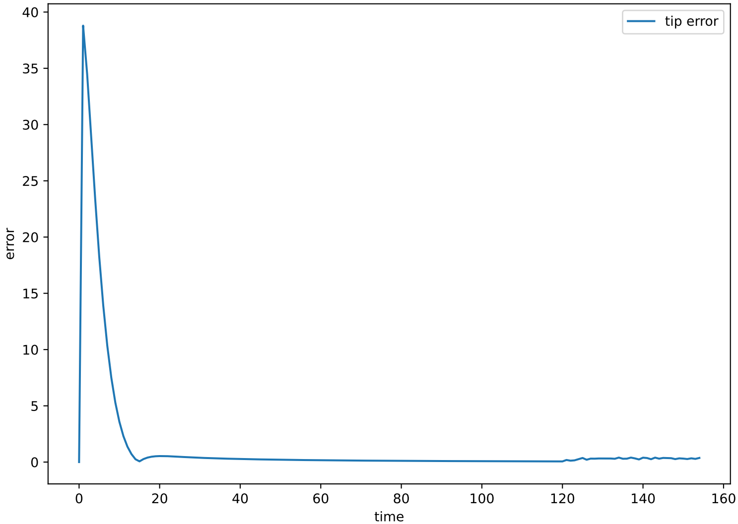
Tip tracking error (replay)
