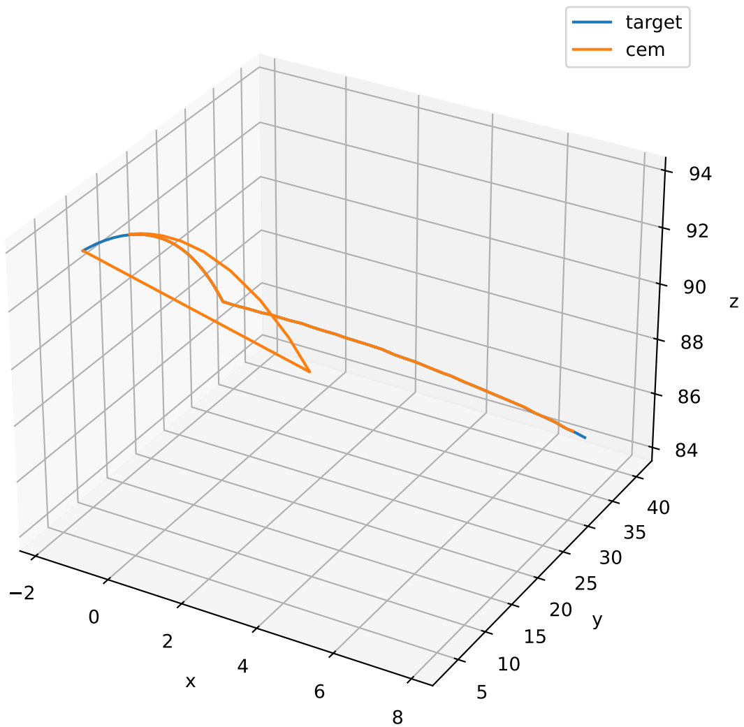
Tip trajectory (replay)
