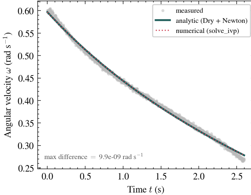
Figure 5: Analytic solution versus direct numerical integration for the slow slam. The curves are indistinguishable (maximum difference \sim 10^{-8} rad/s).
