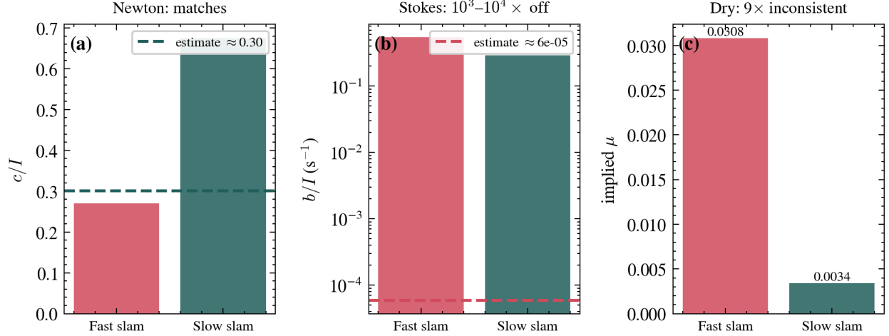
Figure 6: Fitted coefficients against their physical estimates. The Newtonian c/I lands on the predicted value; the Stokes b/I overshoots by three to four orders of magnitude; and the dry-friction coefficient implies two incompatible values of \mu .
