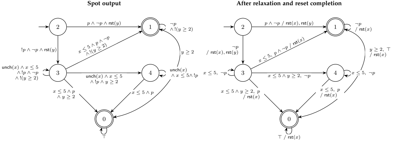
Fig. 4. Spot 2.16 output (TikZ redraw, left; raw DOT and input in examples/spot/ ) and hand-derived reset-completed TBA (right; same state IDs). Here p = \text{LAct}(p) , \neg p = \text{LNAct}(p) , and !p is the literal negation of \text{LAct}(p) . Timed semantics makes !p and \neg p redundant action exclusions; duplicate exclusions are suppressed, while p \wedge \neg p remains for the later TBA simplification. Edges on the right are labeled “guard, action / resets.”
