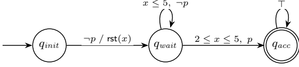
Fig. 3. A hand-simplified equivalent event-guarded TBA for f . The initial transition requires \neg p and resets x . In the waiting location, every outgoing transition checks x \leq 5 ; the transition to the accepting location also requires 2 \leq x . Thus p can first hold only at an event whose age from the origin is in [2, 5] .
