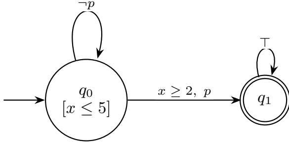
Fig. 3. A two-location TBA for f . The first location enforces the deadline x \leq 5 and the guard x \geq 2 requires p only in the interval [2, 5] .
