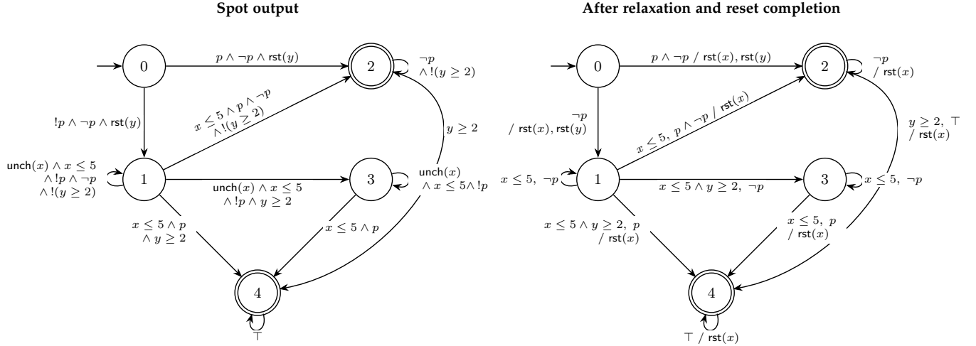
Fig. 4. Generated automata for the worked formula. Left: Spot's Büchi automaton, before timed reinterpretation. Right: after relaxation and reset completion. Here !p is the negative literal of the extended atom p , whereas \neg p is an action proposition; their conjunction is retained until the separate TBA optimization stage. Edges on the right are labeled "guard, action / resets."
