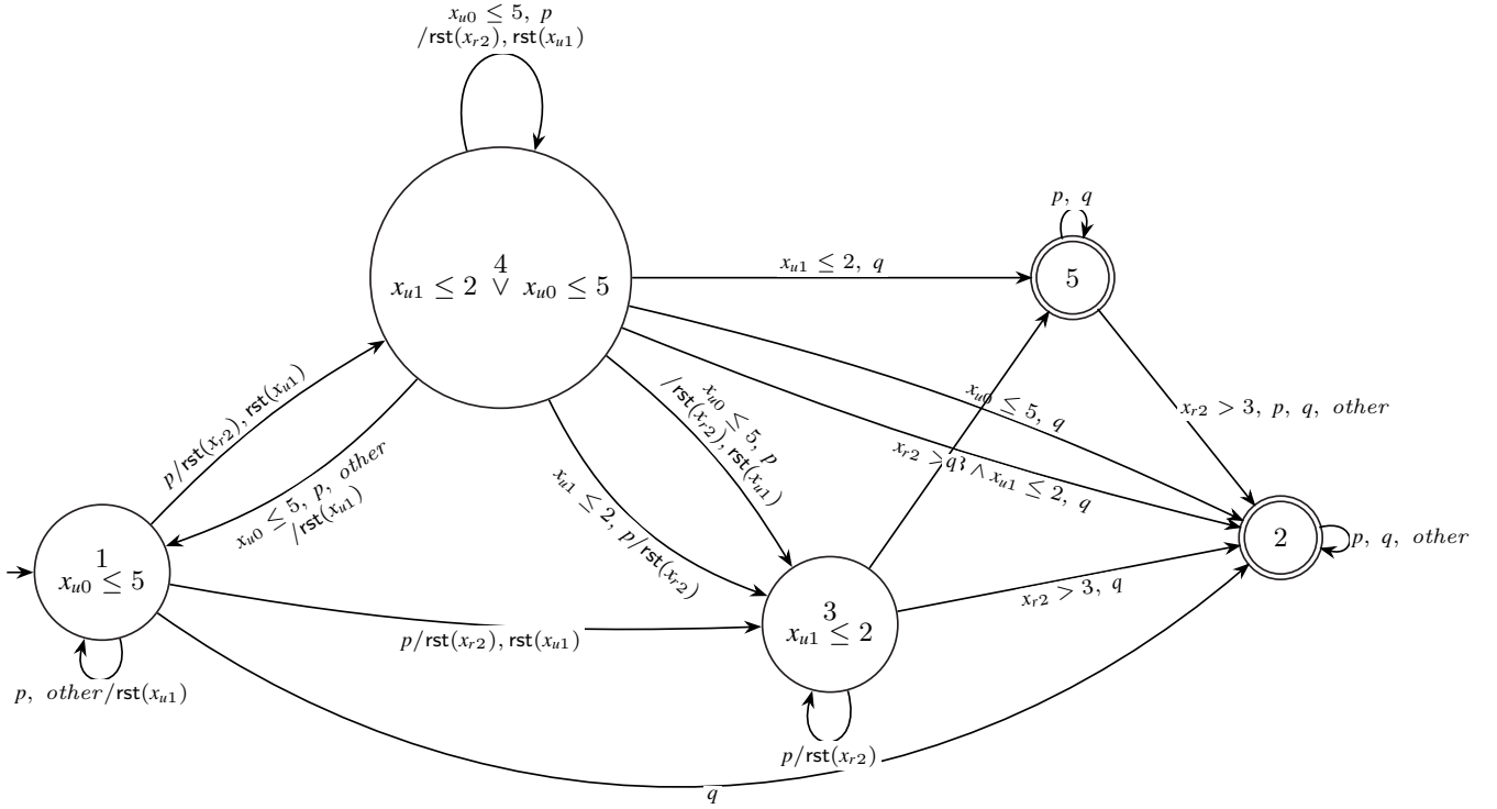
FIGURE 5. Optimized automaton for \Diamond_{\leq 5}((\Box_{\leq 3}(p \vee q)) \cup_{\leq 2} q) before disjunctive-invariant elimination. Clocks x_{u0} , x_{u1} , and x_{r2} belong to the three distinct primitive timed subformulas. The diagram is after the initial _init_ transition; guards implied by source invariants are omitted. A comma-separated event list denotes separate transitions. The q -edges from locations 4 and 3 with x_{r2} > 3 are unsatisfiable for the reasons given in the text.
