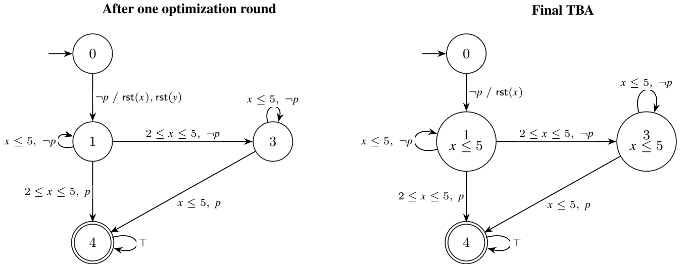
FIGURE 6. F11 after one optimization round and after UPPAAL-oriented export. The first panel shows the removed unreachable location and the two synchronously reset clocks; the final panel shows the merged clock and synthesized invariants. Edges use the form “guard, action / resets,” and the double circle marks the accepting location.
