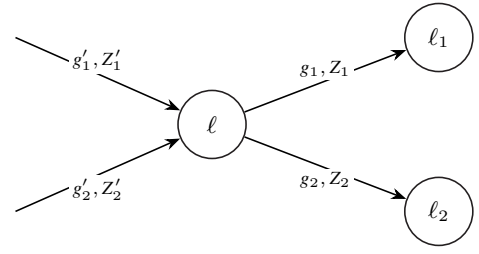
FIGURE 1. Invariant computation. Successor invariants strengthen outgoing guards; upper bounds of the resulting guards resynthesize the source invariant. Reset sets determine which target-clock constraints become constant.
