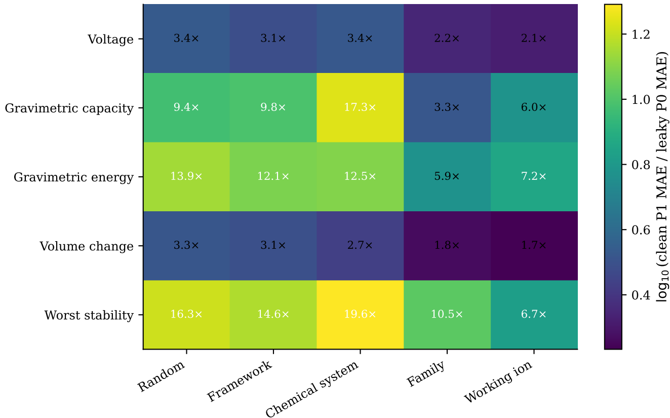
Performance optimism from post-hoc leakage across validation regimes
