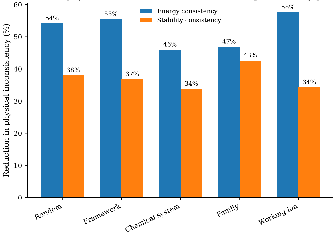
Value of soft physics constraints under the clean composition-only protocol
