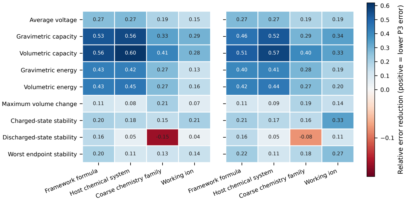
(a) P1 to P3 relative MAE improvement (b) P1 to P3 relative RMSE improvement
