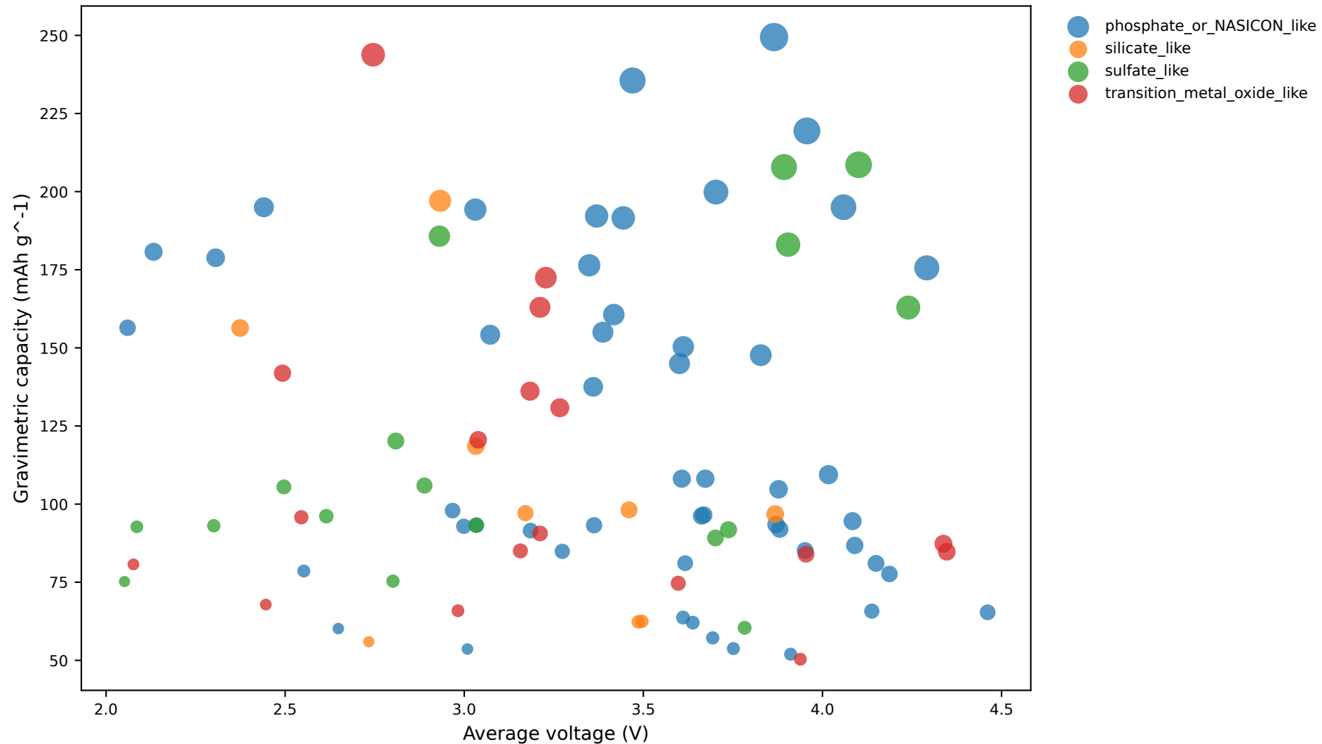
Figure 5. Candidate voltage-capacity-energy landscape
