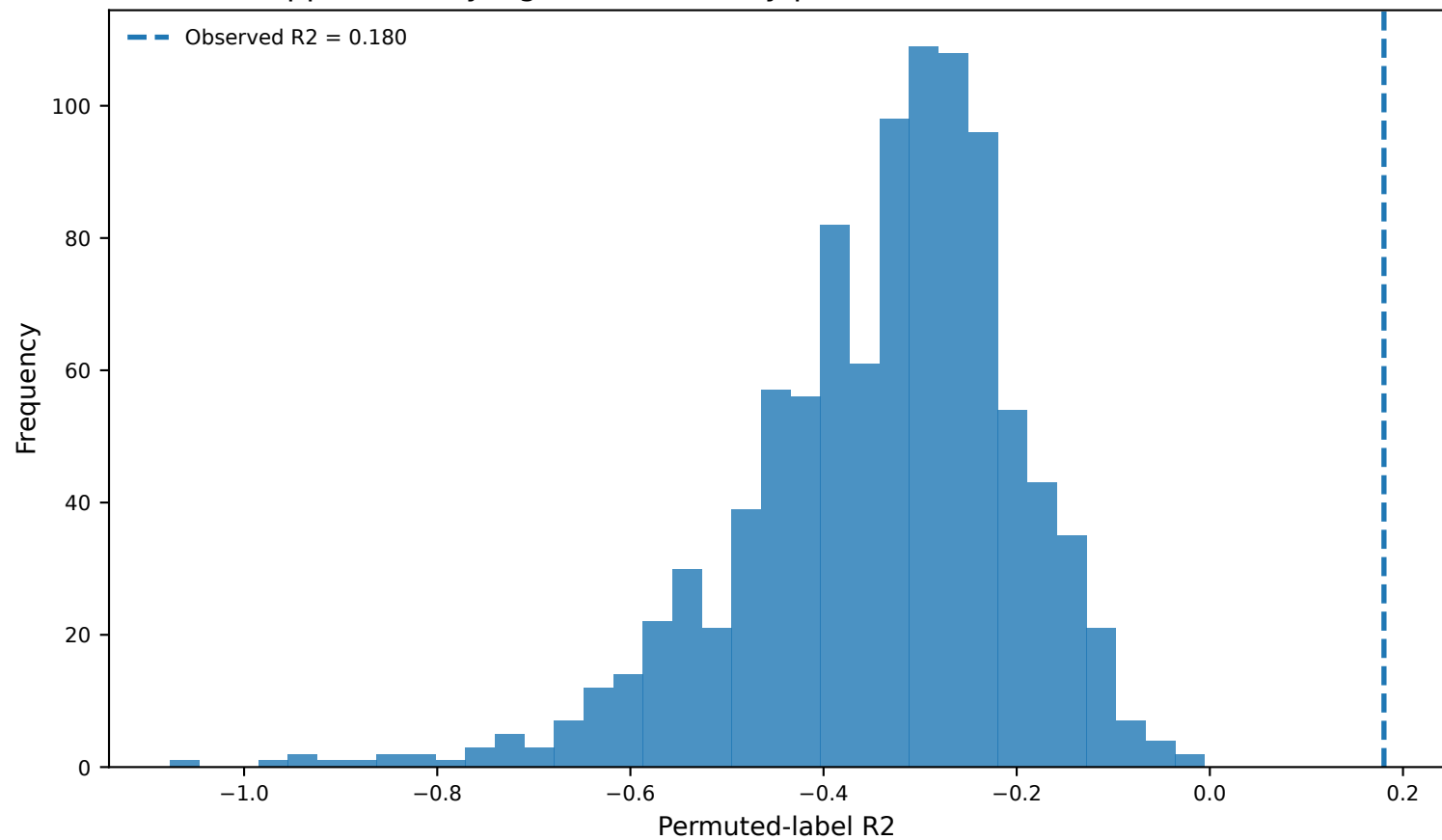
Supplementary Figure S1. Stability permutation-test null distribution
