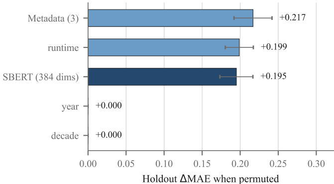
(b) Permutation loss, chronological holdout
