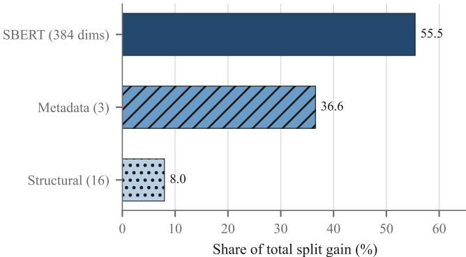
(a) In-sample gain, random split
