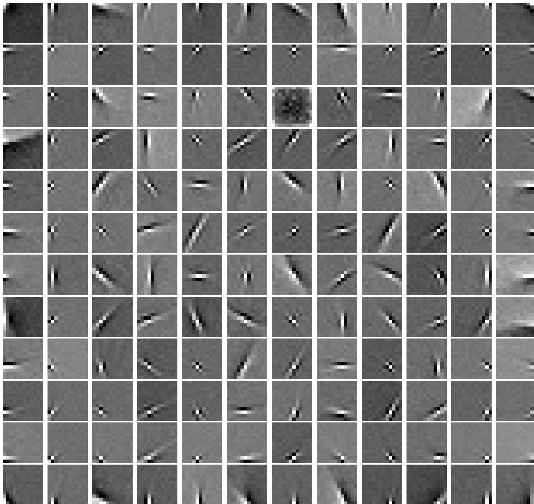
Spatial Receptive Filters Learned from Natural Scenes ( \ell_1 -Domain)
