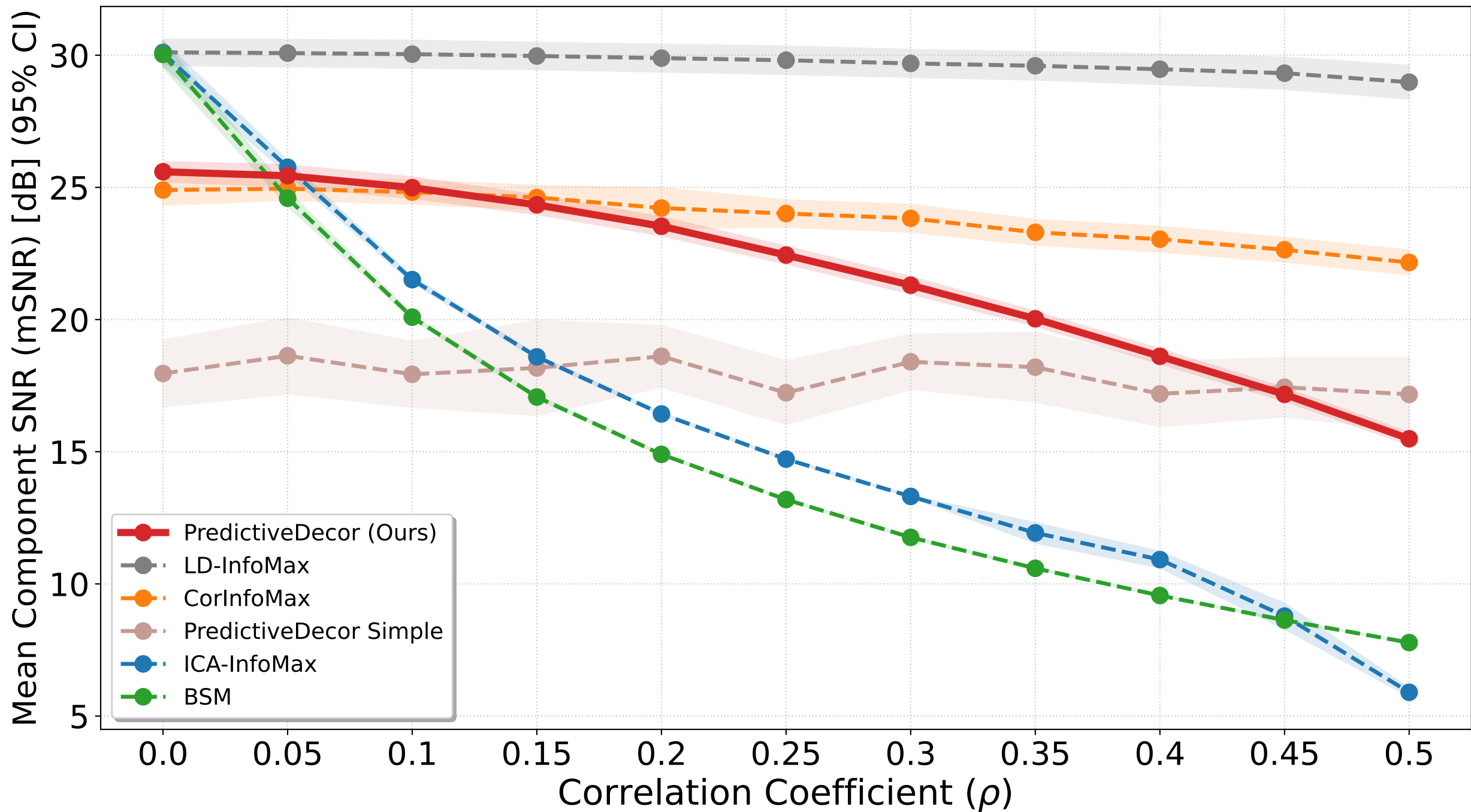
Correlated Antisparsity Source Separation - mSNR Results
