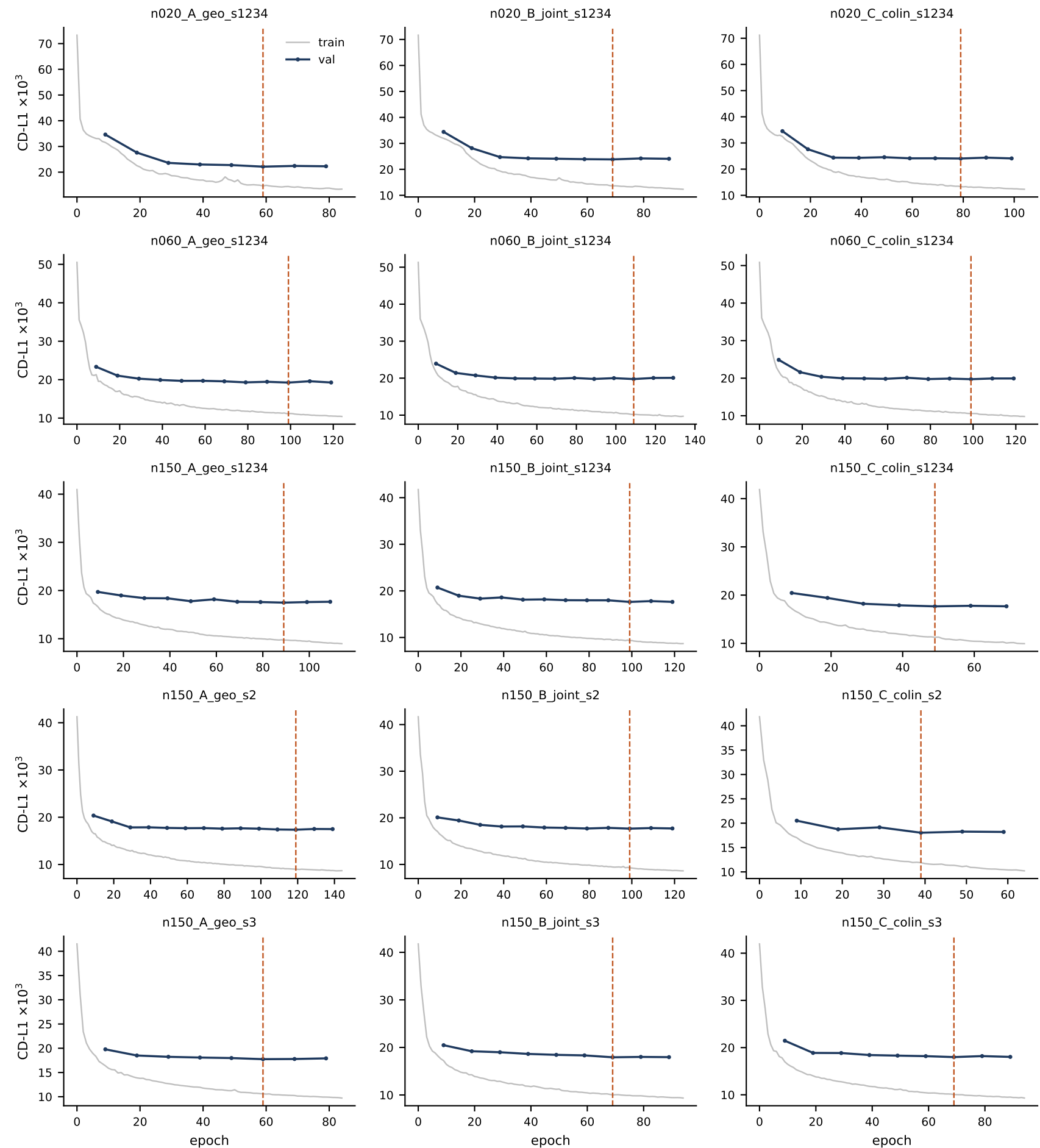
All 15 runs: train/val CD-L1 per epoch (dashed line = best epoch kept by early stopping)
