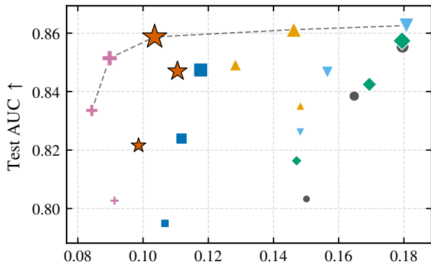
Communities & Crime
