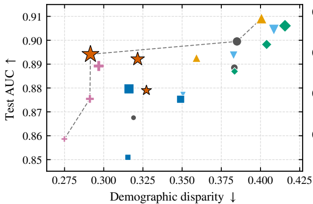
Communities & Crime
