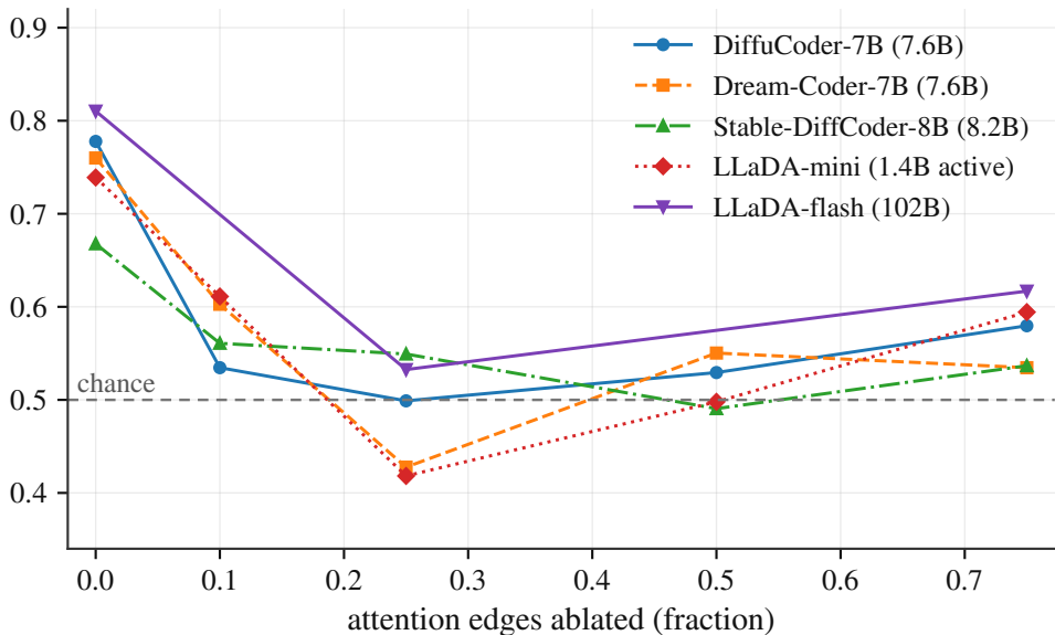
correctness read AUC
