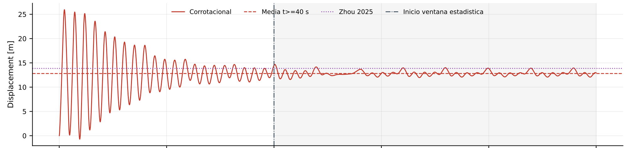
(b) Edgewise tip deflection
