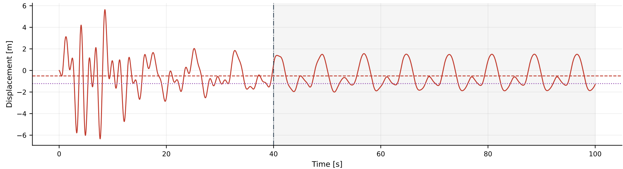
(b) Edgewise tip deflection
