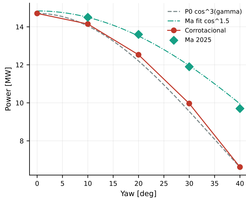
(b) Mean power
