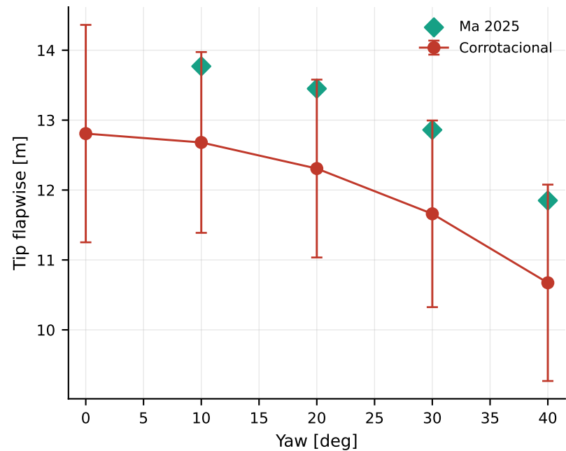
(c) Tip flapwise
