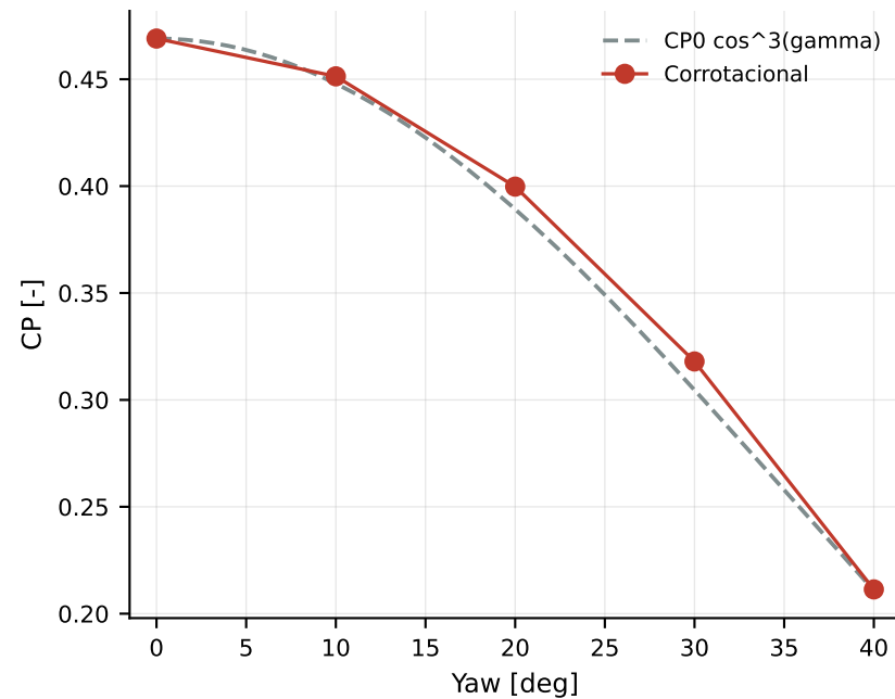
(a) CP vs yaw
