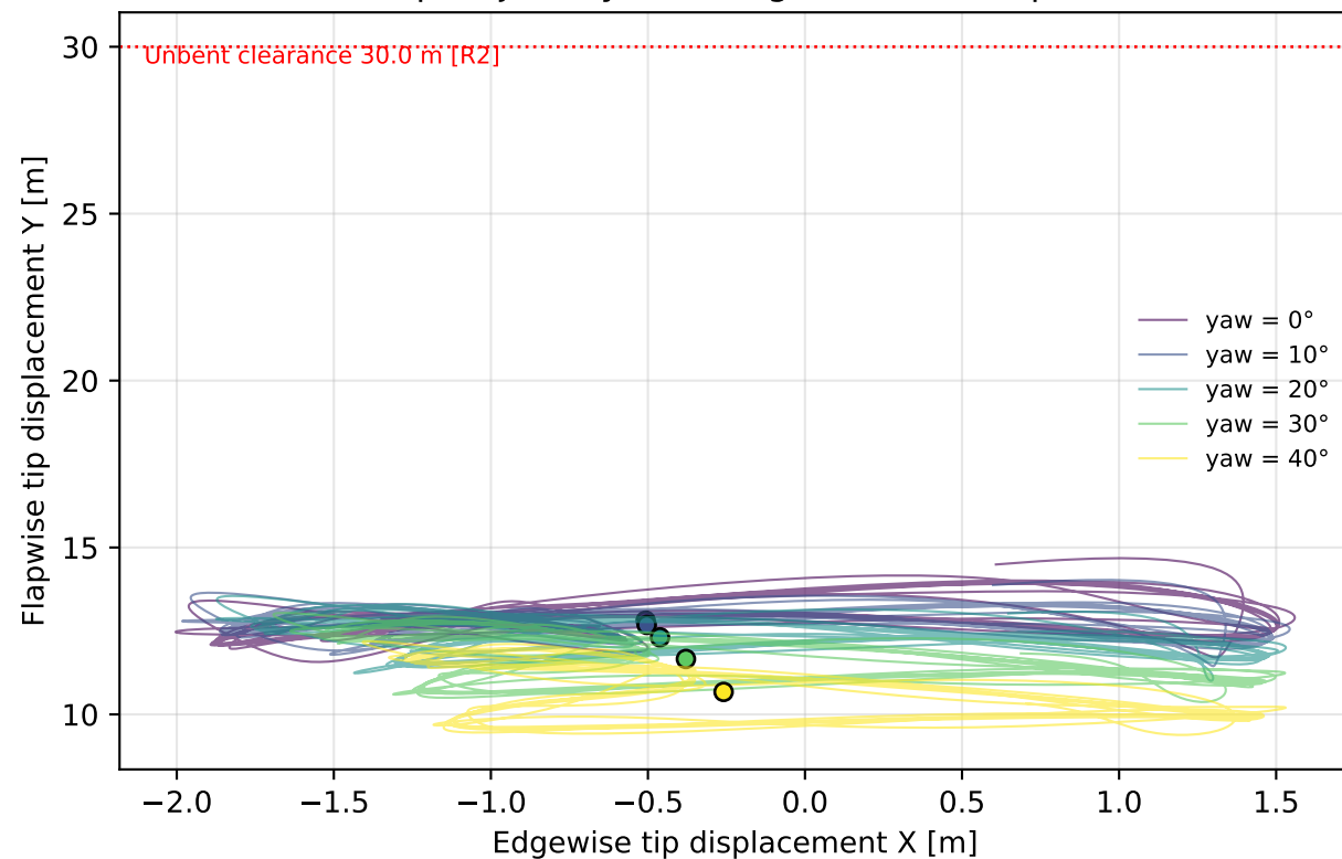
(a) Tip trajectory (X = edgewise, Y = flapwise)
