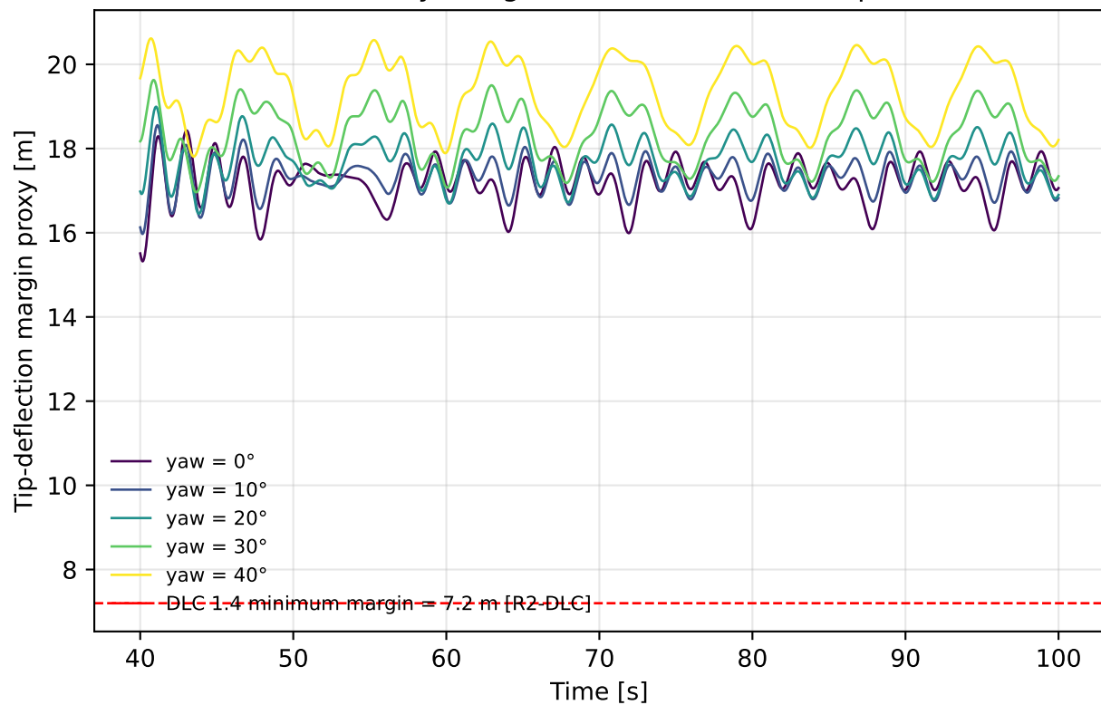
(b) Proxy margin vs. NREL DLC envelope
