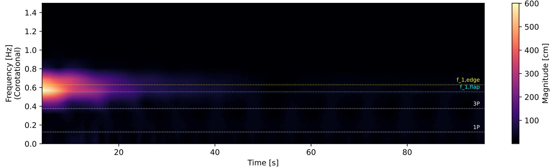
Fixed-tip flapwise displacement spectrogram — IEA 15 MW, yaw=0°, rated STFT (Hann, 8 s window, 87% overlap)
