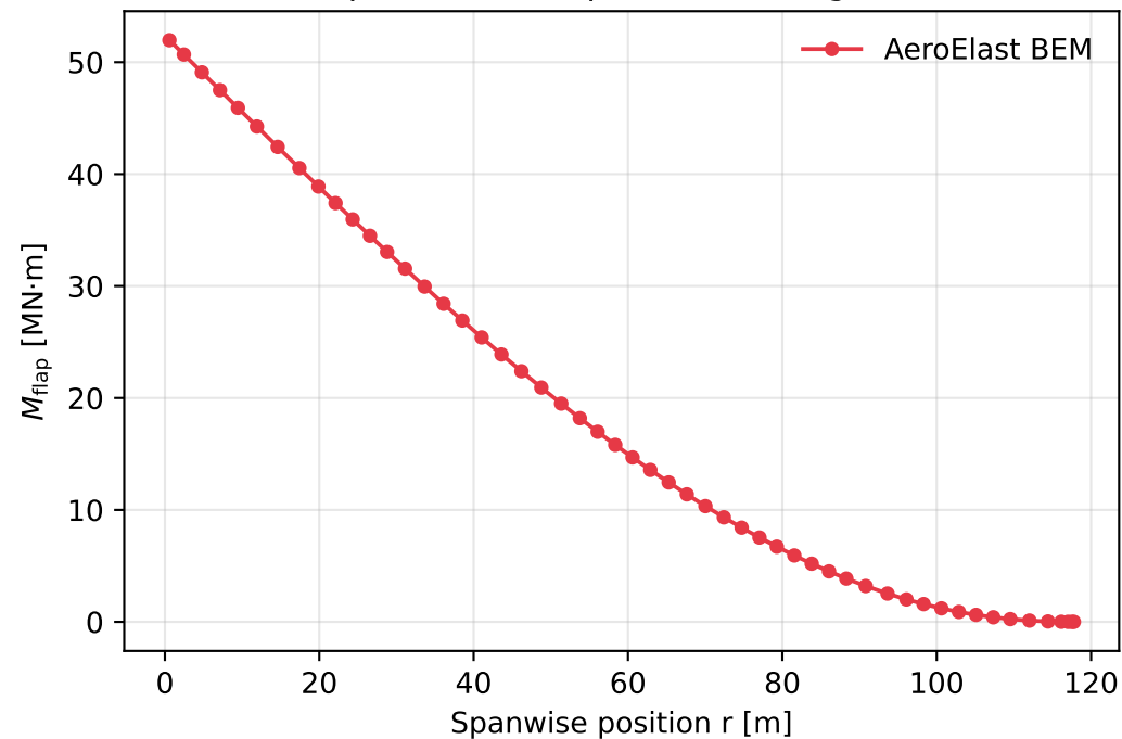
(a) Flapwise (out-of-plane) bending moment
