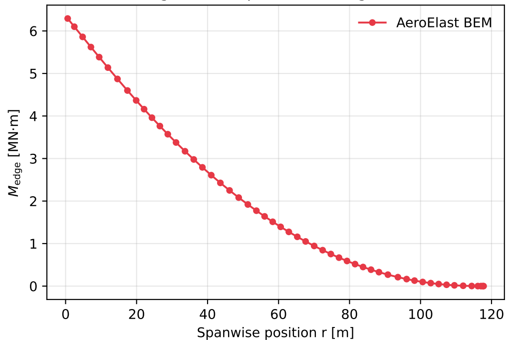
(b) Edgewise (in-plane) bending moment
