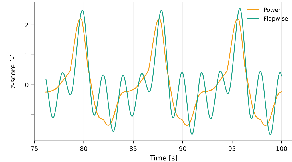
(c) Steady-state normalized power and flapwise
